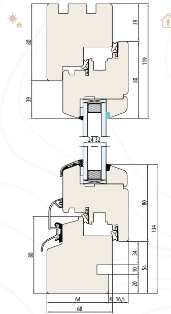
NATURRO 68 SYSTEM The undercut for the interior window sill
