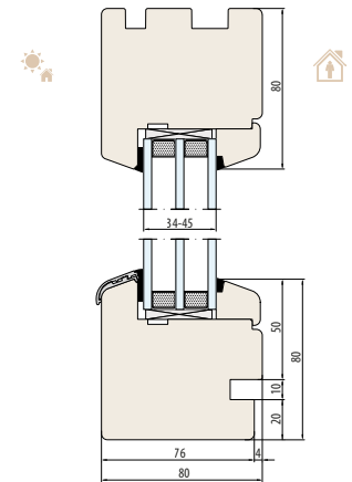
NATURO 80 - FIX SYSTEM The undercut for the interior window sill
