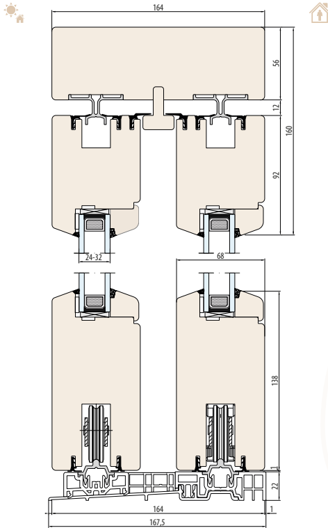
NATURO 68 HST SYSTEM (general dimensions) - threshold 22 mm - scheme 'D'
