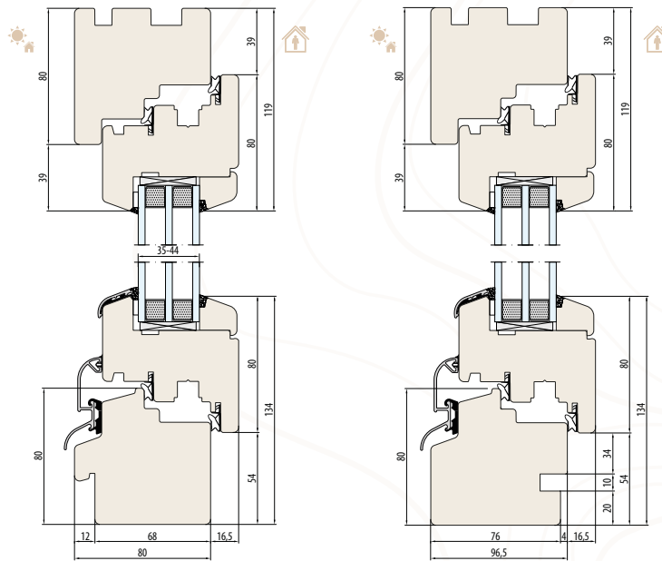
NATURO 80 SYSTEM The undercut for the exterior window sill
