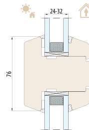
NATURO 68 SYSTEM Muntin bar 76 mm
