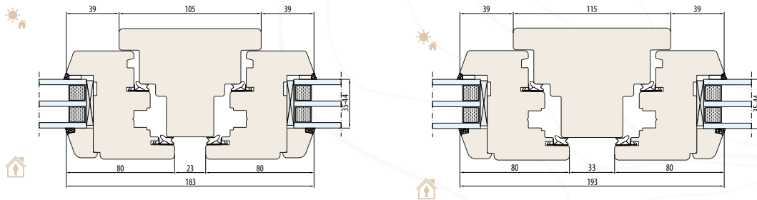
NATURO 80 SYSTEM fixed post 105 mm (Horizontal cross-section)
