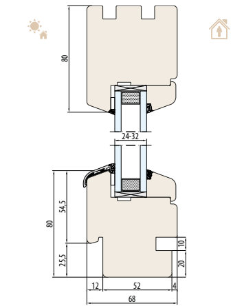
NATURO 68 - FIX SYSTEM The undercut for the interior and exterior window sill
