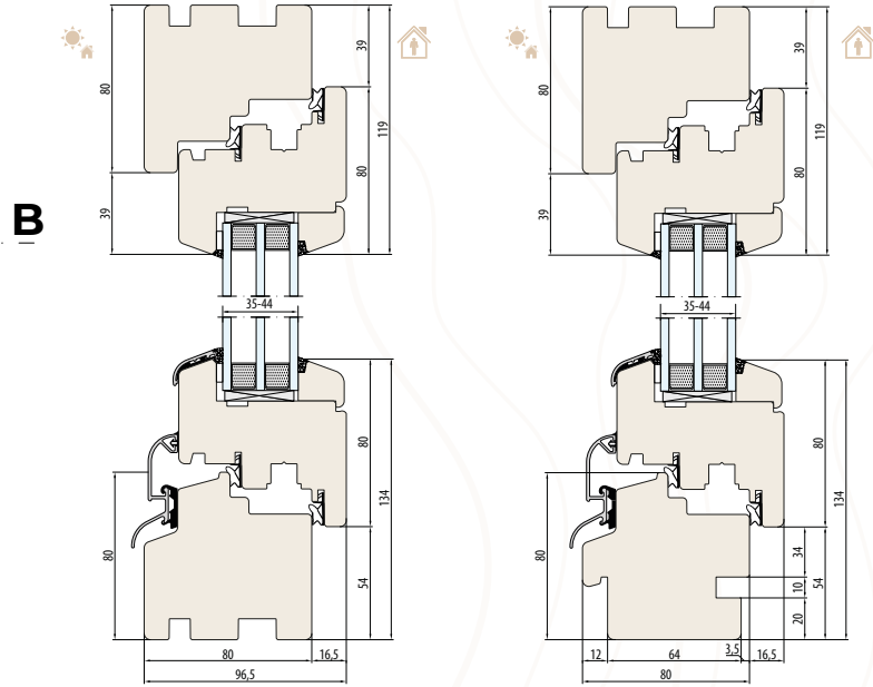
NATURO 80 SYSTEM Without undercut for the window sill
