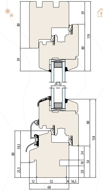
NATURRO 68 SYSTEM The undercut for the interior and exterior window sill
