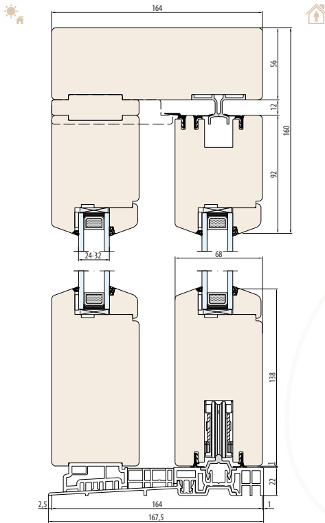
NATURO 68 HST SYSTEM (general dimensions) - threshold 22 mm - scheme 'A'
