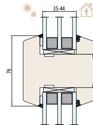
NATURRO 80 SYSTEM Muntin bars 76 mm
