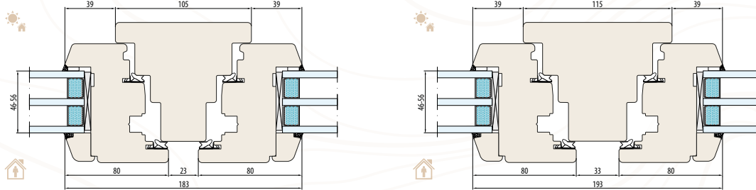
NATURO 92 SYSTEM fixed post 105 mm (Horizontal cross-section)
