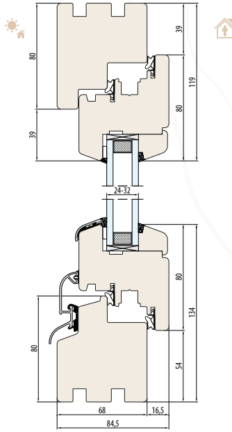
NATURRO 68 SYSTEM Without undercut for the window sill
