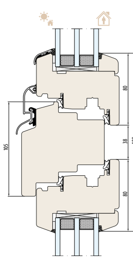
NATURO 92 SYSTEM transom bar 105 mm
