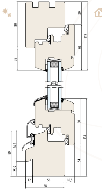
NATURRO 68 SYSTEM The undercut for the exterior window sill
