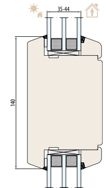
NATURRO 80 SYSTEM Muntin bars 140 mm
