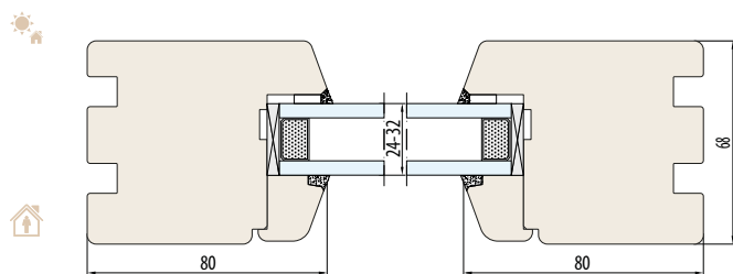
NATURO 68 - FIX SYSTEM HORIZONTAL CROSS-SECTION B-B
