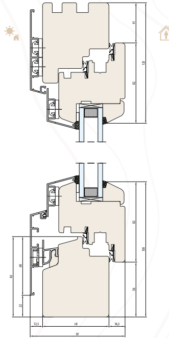
SYSTEM NATURO 68 ALU RENO LINE Without undercut for the window sill
