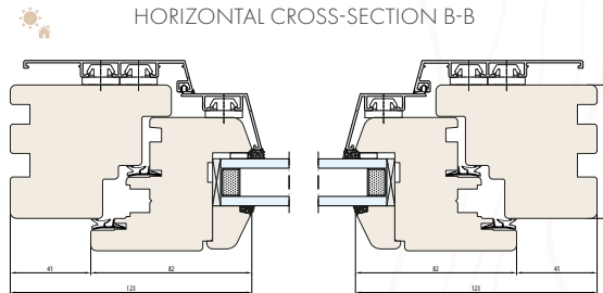
SYSTEM NATURO 68 ALU RENO LINE
