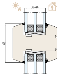
NATURRO 80 SYSTEM Muntin bars 68 mm
