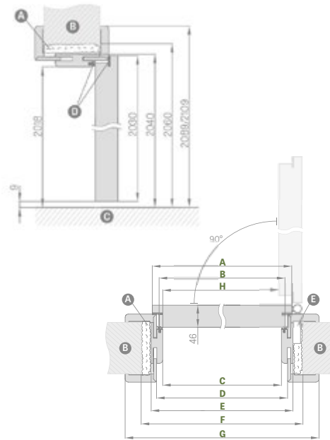
Scheme of the adjustable door frame
