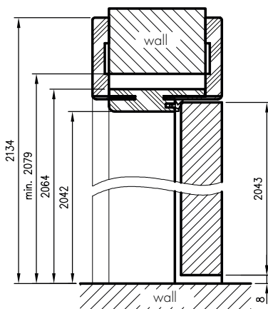
Vertical cross-section of non-rebated doors in ORB
