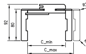
Cross-section of ORB 075
