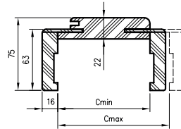
OR/ORC section with angle.T63
