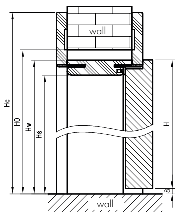
Vertical section OR
