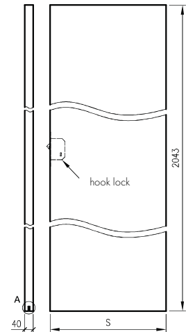
Sliding sashes for: - PA door frame cassettes - SPAZIO CD systems - wall systems
