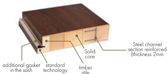
SECTION OF HERSE SASH 32 DB
