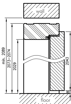
OP VERTICAL SECTION FOR REBATED DOORS
