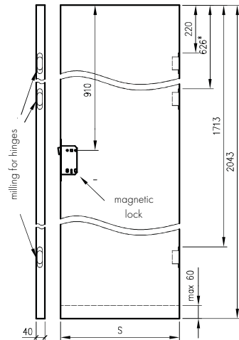
Non-rebated turn sashes
