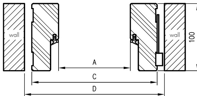
Horizontal section of the OPB
