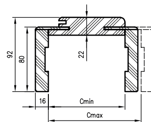
OR horizontal section
