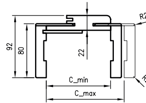
Cross-section of ORB 095-300
