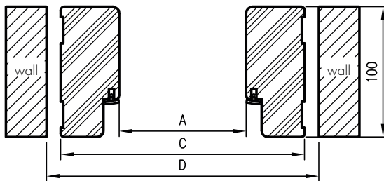
Dimensions for single-sash doors
