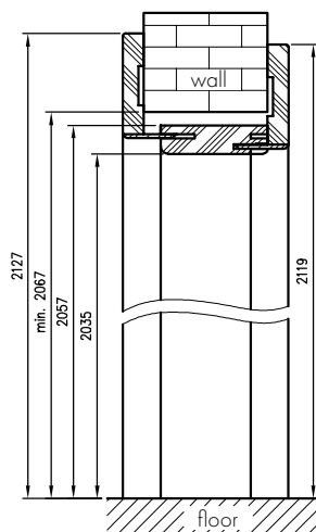
Vertical section of the adjustable tunnel with an angle. T80
