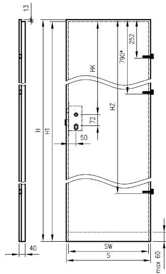
Non-rebated door sashes: Standard 10, Modern, Plus
