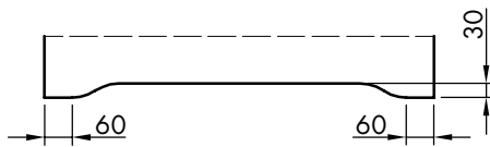
standard undercut in the door
