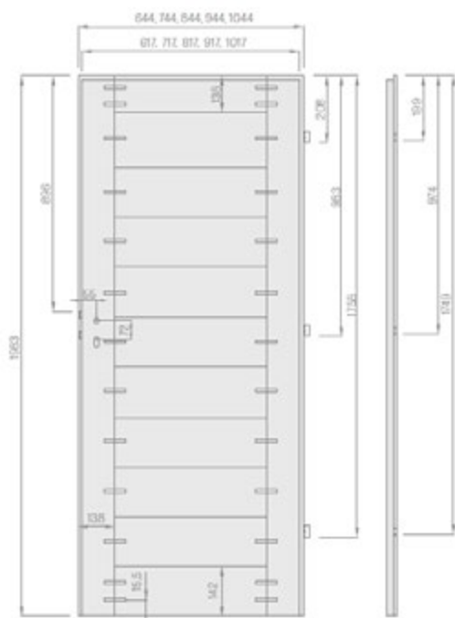
Rebated door sash
