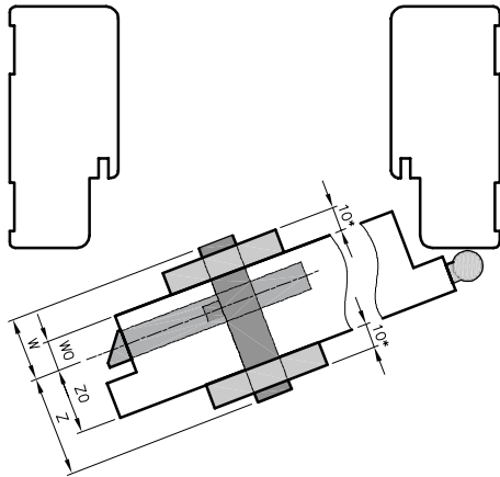
Fig. Selection of cylinder insert dimensions
