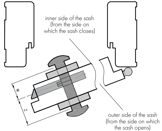
Fig. Selection of cylinder dimensions with a knob
