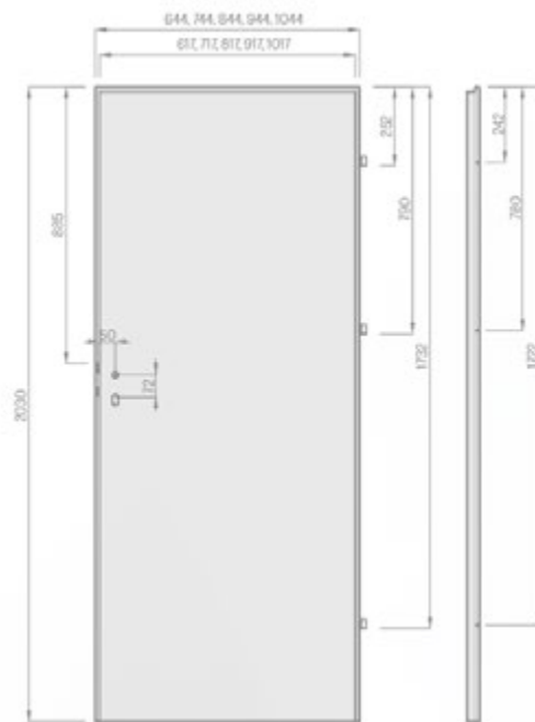
Rebated door sash
