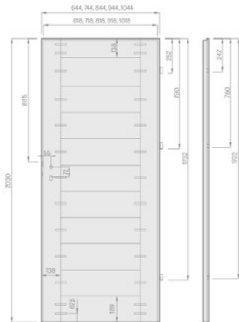
Rebated door sash
