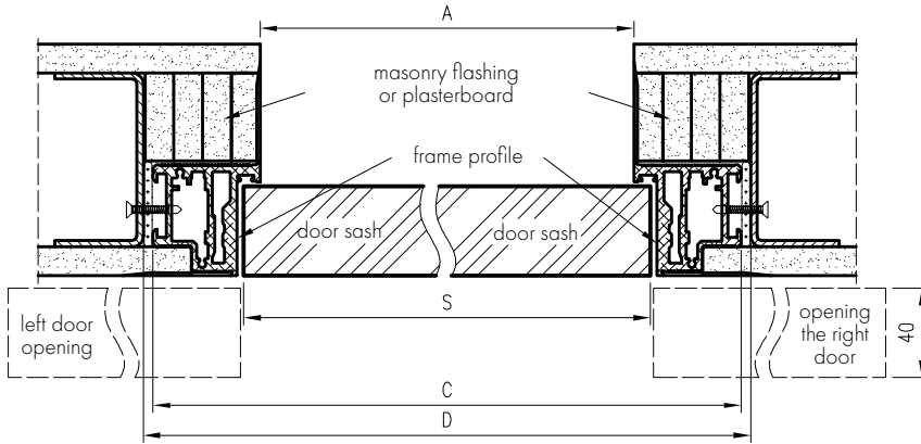
Cross-section of the Sara Eco2 non-rebated door - opened outwards
