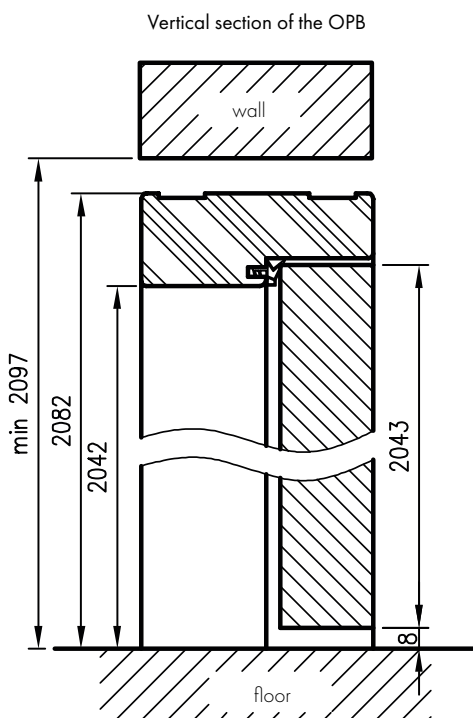
For single-sash doors
