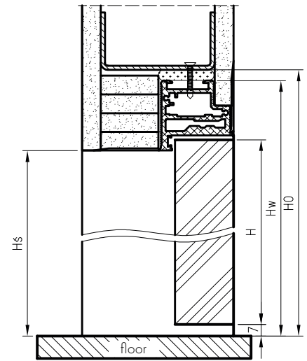
Vertical section of the Sara Eco 2 non-rebated door - opened outwards
