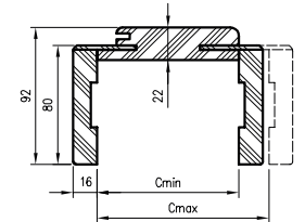
OR/ORC section with angle.T80
