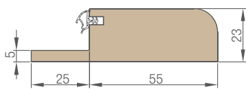
Hardwood threshold
