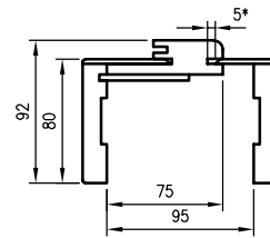
Section of ORB 075
