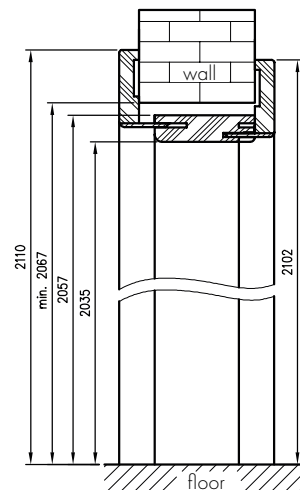
Vertical section of the adjustable tunnel with an angle. T63
