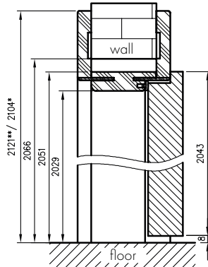
Vertical section of the rebated door with OR
