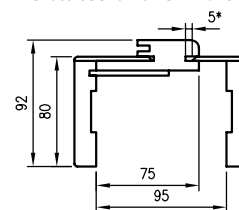
Cross-section of ORB 075
