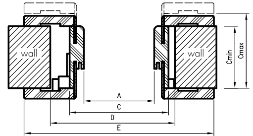
horizontal section ORB
