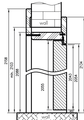
Vertical section ORO
