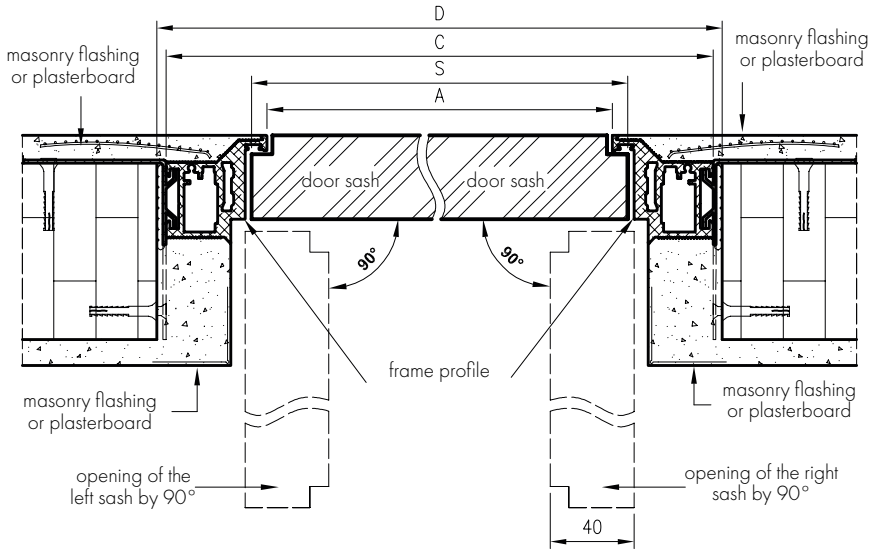
Cross-section of the Sara Eco2 rebated door - opening inwards
