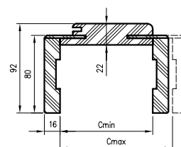
OR/ORC section with angle.T80
