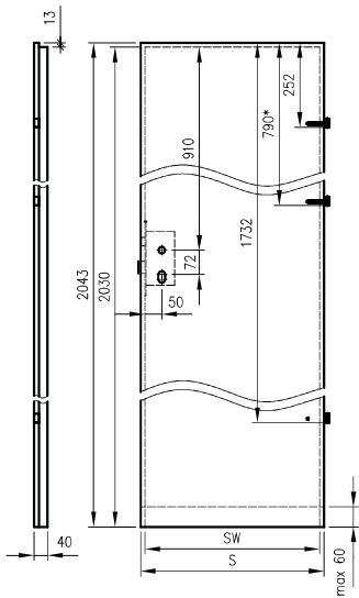
Non-rebated turn sashes
