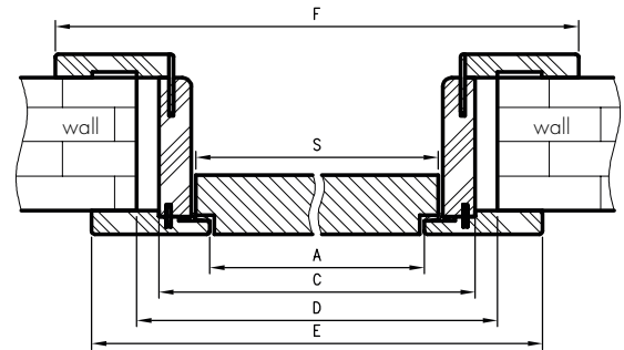
Cross-section of ORO
