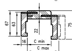
TUN section with angle. T63
