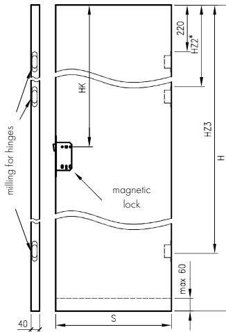
Non-rebated door sashes: Standard 10, Modern, Plus
