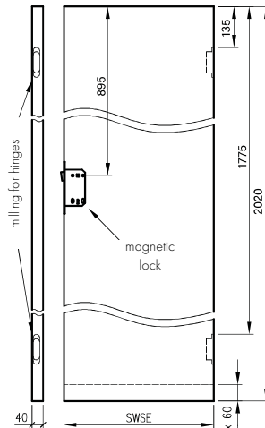
Sara Eco 2 non-rebated door sashes in the 202X standard
