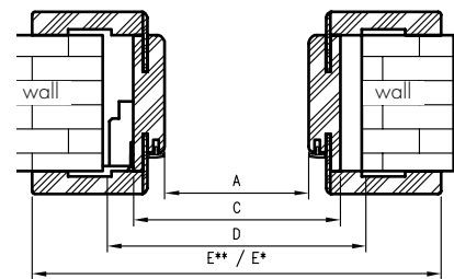
OR/ORC horizontal section
