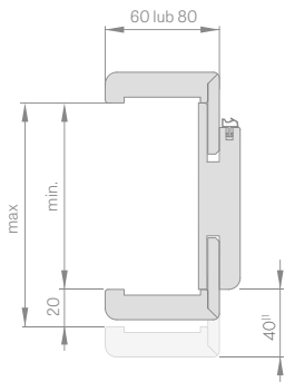
Adjustment range of the adjustable door frame
