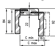
TUN section with angle. T80
