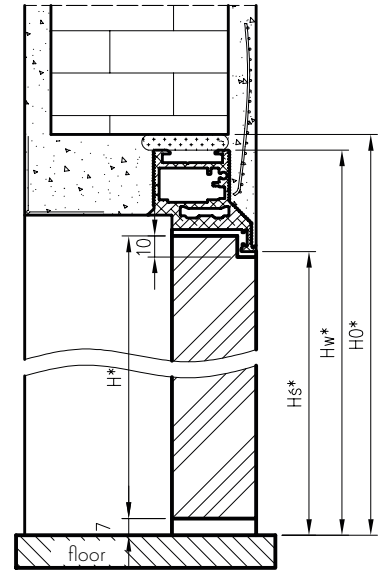
Cross-section of the Sara Eco2 rebated door - opening inwards
