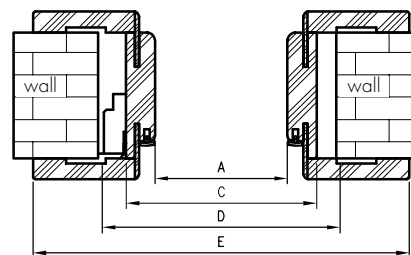
OR horizontal section
