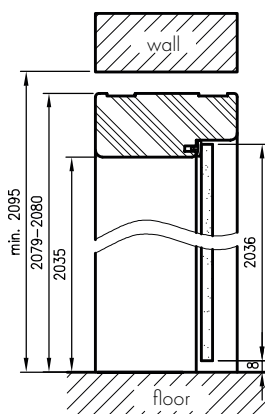
OP VERTICAL SECTION FOR GLASS DOORS
