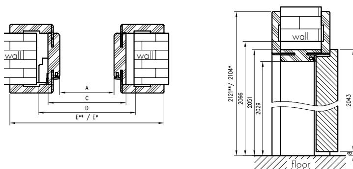
Dimensions for single-sash doors
