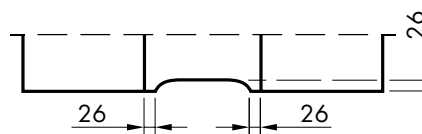
undercut in the Vetro B door
